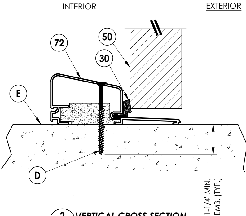
2 5 VERTICAL CROSS SECTION Shown w/ High Dam Threshold
