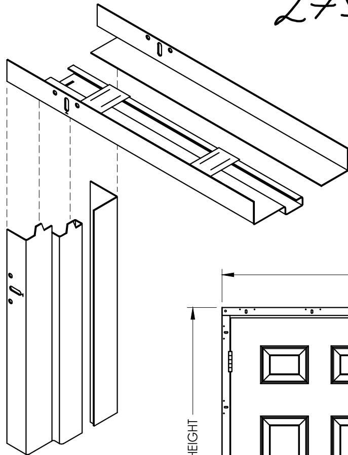
REDIFLEX TWO-PIECE
