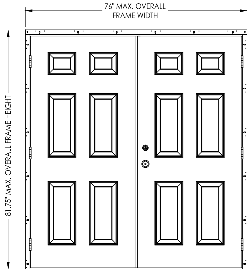
OUTSWING
